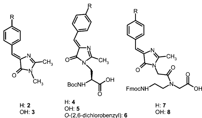
Figure 2. GFP chromophores 2 and 3 and their incorporation into alaninyl derivatives 4–6 and N -(2-aminoethyl)glycinyl amino acids 7 and 8 .
