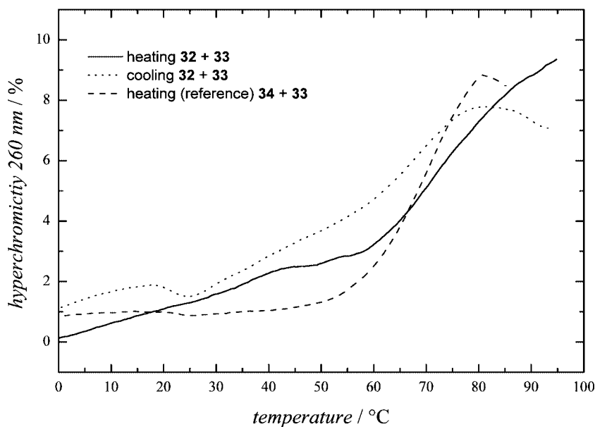
Figure 7. UV melting curve of oligomer 32 after hybridization with complementary DNA 33 (5'-G-C 2 -G-C 2 -A 5 -3'), each 3 \mu\text{M} in 10 mM \text{NaH}_2\text{PO}_4 buffer, 0.1 M NaCl, pH 6.85. The binding of Uronium-t-t-t-t-g-g-g-g-c-Lys-Lys-Gly-NH 2 ( 34 ) with DNA 33 is also shown, as a reference. [17]
