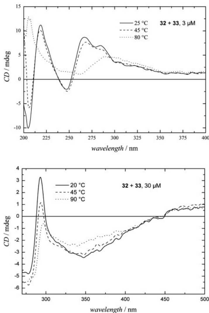
Figure 8. Top : CD spectra of oligomer 32 after hybridization with complementary DNA 33 , each 3 \mu M in 10 mM \text{NaH}_2\text{PO}_4 buffer, 0.1 M NaCl, pH 6.85. Bottom : Same pairing complex, but oligomer and DNA each 30 \mu M in the same buffer. The concentration needed to be increased for monitoring of the CD effect at the optical transitions of the (H)GFP chromophore since its absorption coefficient ( \epsilon_{350\text{nm}} \approx 9 \cdot 10^3 \text{ cm}^2 \cdot \text{mol}^{-1} ) is much smaller than that of the double strand ( \epsilon_{260\text{nm}} \approx 206 \cdot 10^3 \text{ cm}^2 \cdot \text{mol}^{-1} ).
