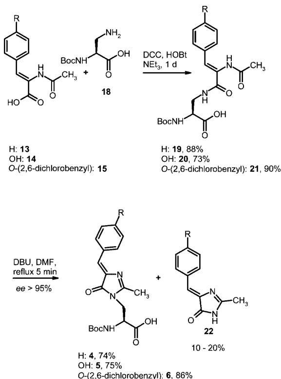
Figure 4. Synthesis of Boc-L-alaninyl GFP chromophores 4–6 .
