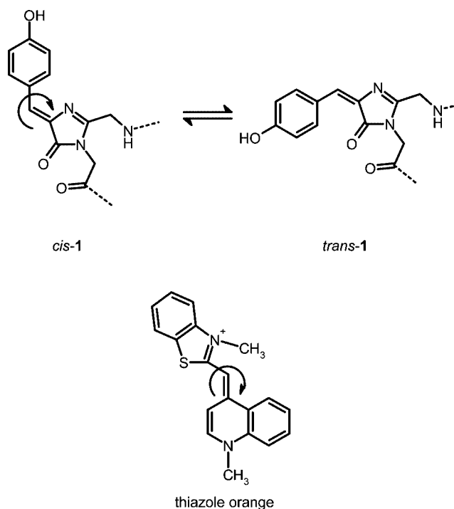
Figure 1. The proposed fluorescence quenching mechanism of the GFP chromophore 1 and comparison with thiazole orange.
