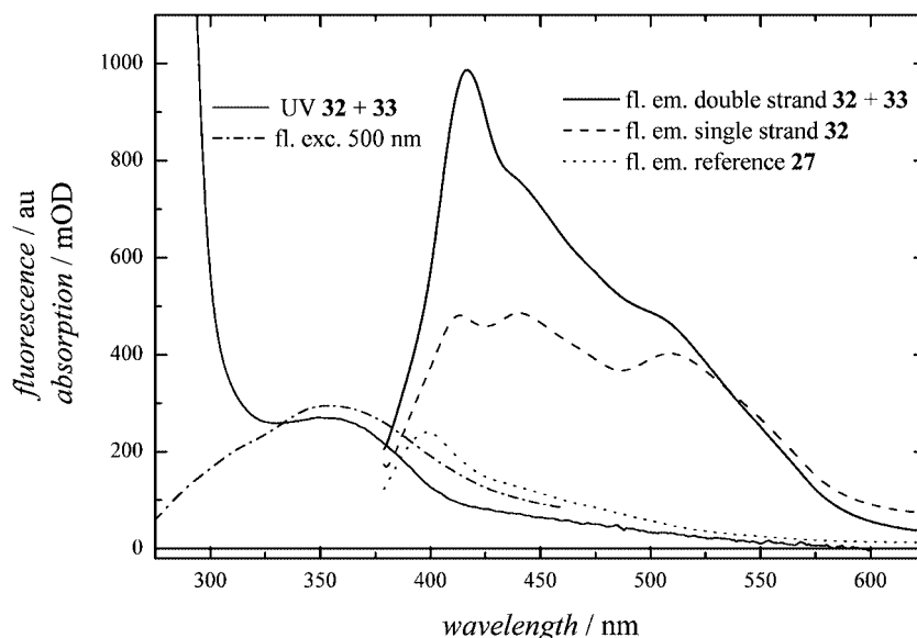
Figure 10. Fluorescence and UV spectra of oligomer 32 depending on hybridization; concentrations of oligomer 32 and DNA 33 each 30 \mu M in 10 mM \text{NaH}_2\text{PO}_4 buffer, 0.1 M NaCl, pH 6.85. UV absorption: \lambda_{\text{max}} = 356 nm; fluorescence emission: \lambda_{\text{exc}} = 350 nm, A_{350\text{nm}} = 0.27 ; single strand \lambda_{\text{em}} = 413, 440, 510 nm, \Phi_{\text{rel}} = 6 ; double strand \Phi_{\text{rel}} = 12 ; reference (H)GFPC-methyl acetate 27 , \lambda_{\text{exc}} = 350 nm, A_{350\text{nm}} = 0.27 in methanol, \lambda_{\text{em}} = 398 nm, \Phi_{\text{rel}} = 1 ; fluorescence excitation: 32 + 33 , \lambda_{\text{em}} = 500 nm (fix), \lambda_{\text{max}} = 356 nm (scanned). A = absorption, \Phi = fluorescence quantum yield.
