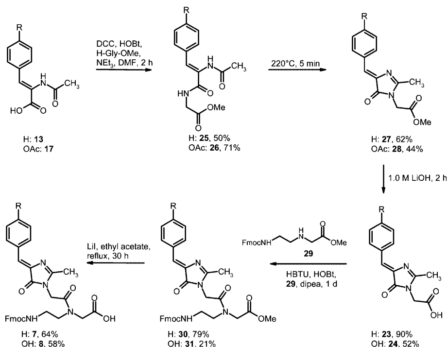
Figure 5. Synthesis of N -(2-aminoethyl)glycine-functionalized GFP chromophores 7 and 8 .
