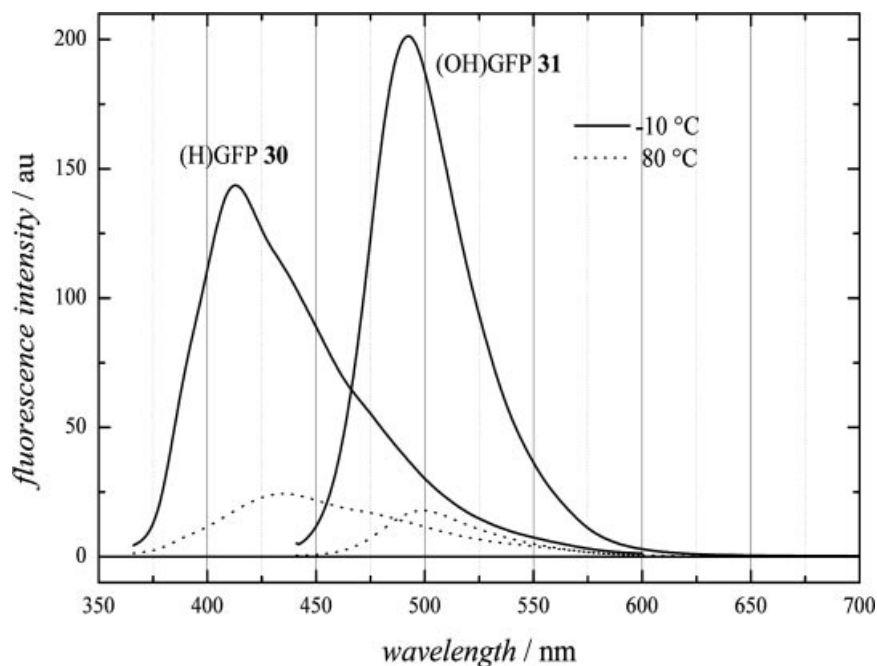
Figure 6. Temperature dependences of the fluorescence emissions of Fmoc-aeg-H(GFPC)-OMe ( 30 ) [ \lambda_{exc} = 350 nm, A_{350\text{nm}} = 0.9 , \lambda_{em} = 436 nm, \Phi_{rel} = 1 (80 °C) and \lambda_{em} = 413 nm, \Phi_{rel} = 5 (–10 °C)] and of Fmoc-aeg-(OH)GFPC-OMe ( 31 ) [ \lambda_{exc} = 430 nm, A_{430\text{nm}} = 1.6 , \lambda_{em} = 499 nm, \Phi_{rel} = 1 (80 °C) and \lambda_{em} = 492 nm, \Phi_{rel} = 11 (–10 °C)] in glycerin (+ 0.1% \text{NEt}_3 for 31 ) at 80 °C and in glycerin glass at –10 °C. A = absorbance; \Phi = fluorescence quantum yield.
