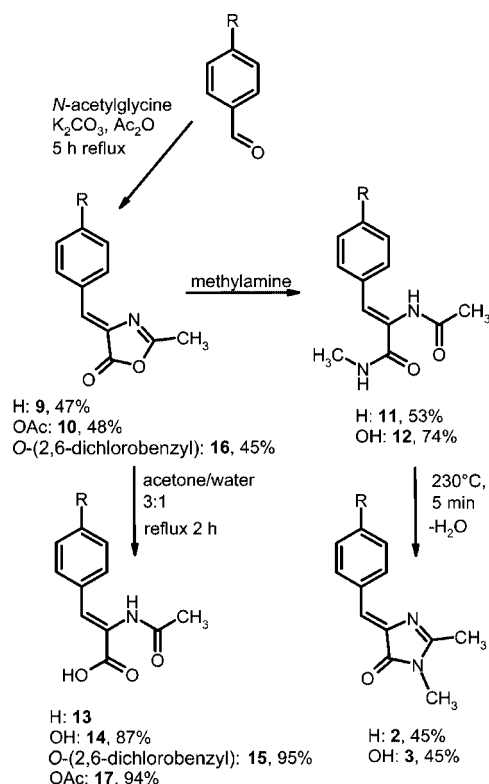
Figure 3. Synthesis of the 3-methyl-GFP chromophores 2 and 3 .
