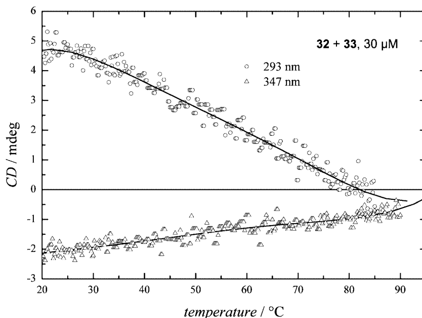
Figure 9. Temperature dependency of the CD effect at the optical transitions of the (H)GFP chromophore at 293 nm and 347 nm. Oligomer 32 + DNA 33 each 30 \mu M in 10 mM \text{NaH}_2\text{PO}_4 buffer, 0.1 M NaCl, pH 6.85.
